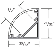
MRSI-CHAN-SLV-6.5 Anodized aluminum extrusion available in 6.5' length
